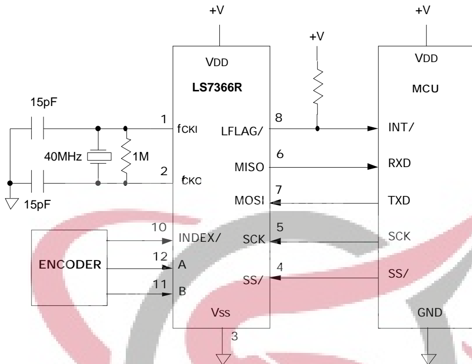
FIGURE 13. GENERAL I/O CONNECTIONS
